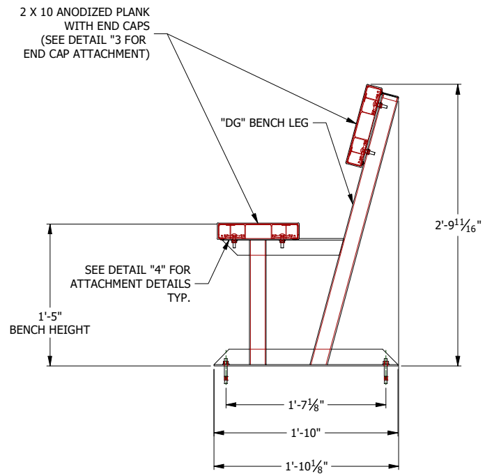
CONCRETE ANCHOR OPTION SEE DETAIL "2"
